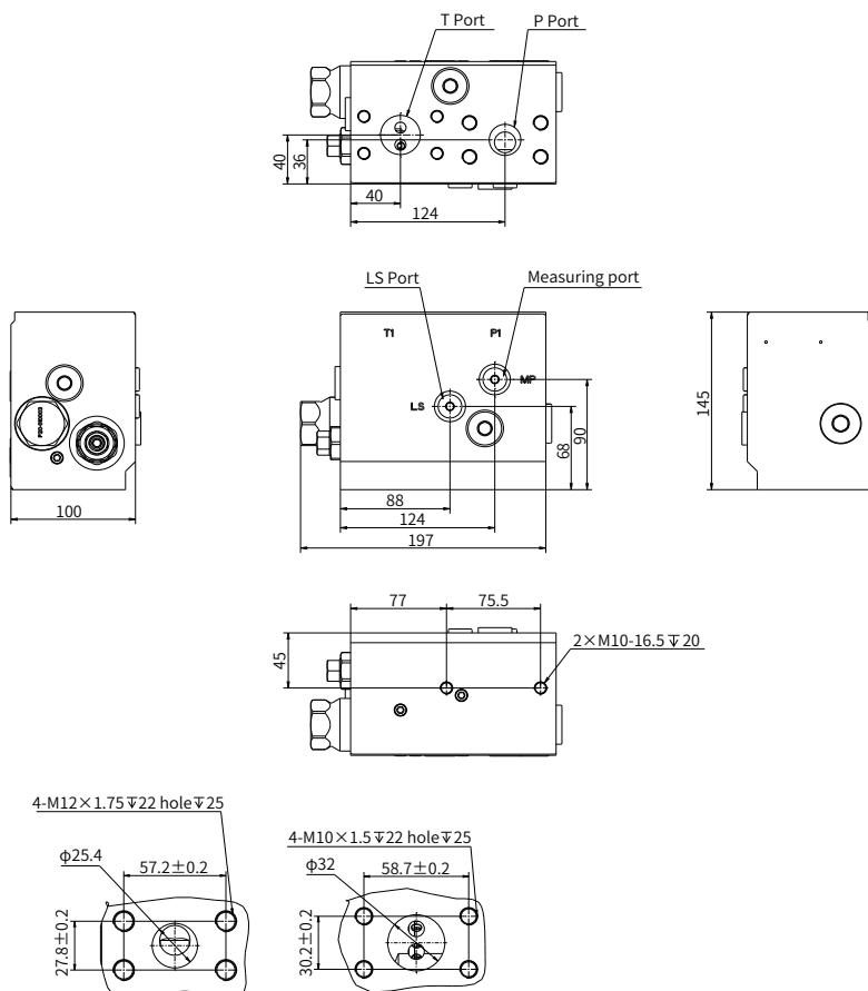
1' port flange interface (high pressure) 1-1/4' port flange interface
