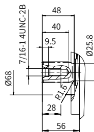
“C2” 型花键轴
